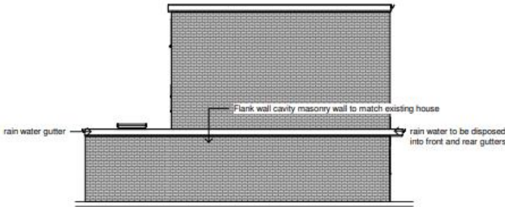
8 Proposed Flank Elevation 1 : 100
