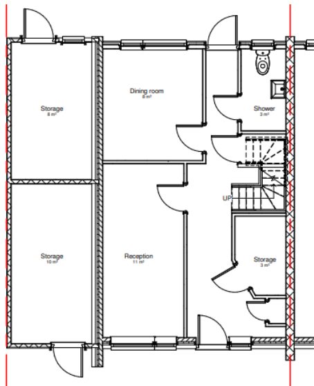
① 00 Existing Ground Floor 1 : 50
