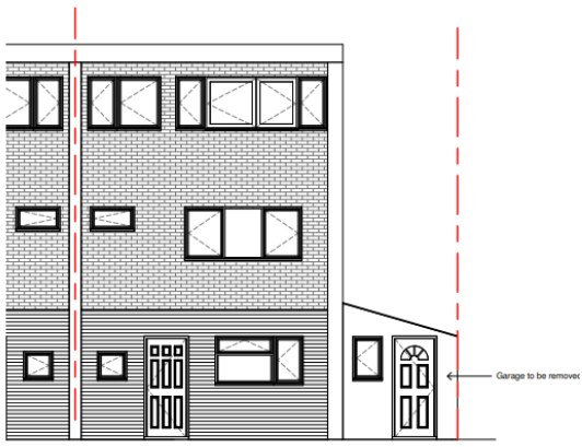
⑥ Existing Rear Elevation 1 : 50
