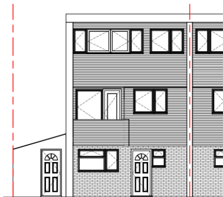
⑤ Existing Front elevation 1 : 50
