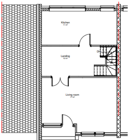
② 01 Existing First Floor 1 : 50
